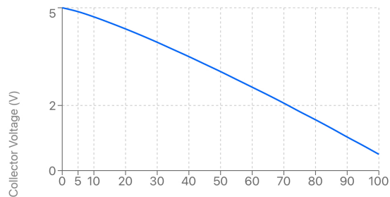
RPR-220 Collector Voltage vs Reflection Percentage
